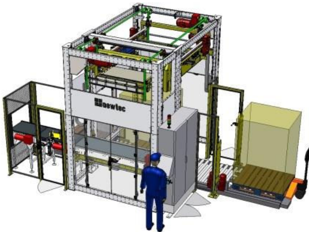
Schematic of Newtec's PAL 500 series/PAL-PACK 3300 palletiser
