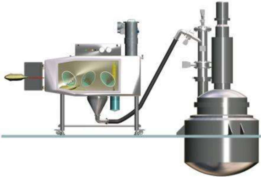
High-containment bag emptying station from Dietrich Engineering Consultants
