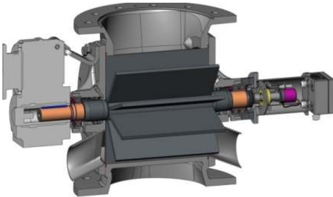
Coperion's compactly built RotorCheck
